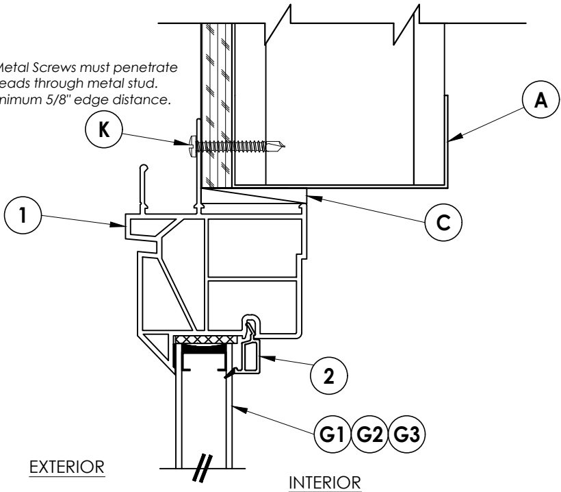
3 VERTICAL CROSS SECTION 3 Shown w/ Steel Stud Framing Option
