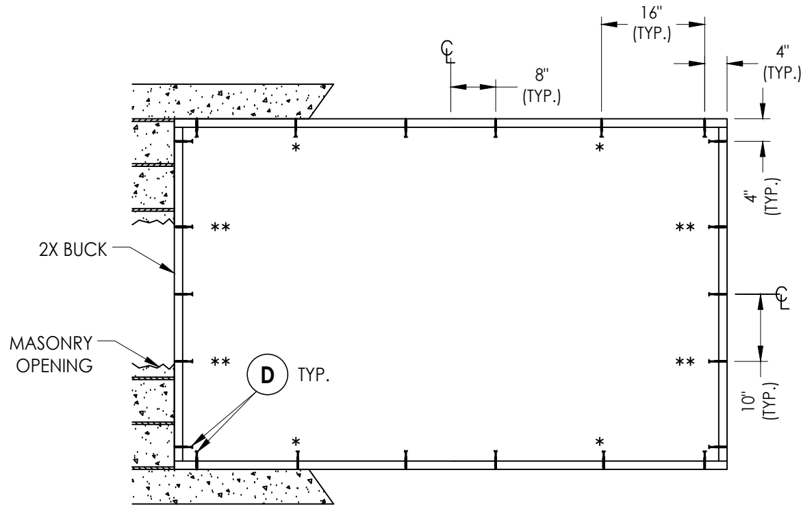
BUCK ANCHORING (2X BUCK)
