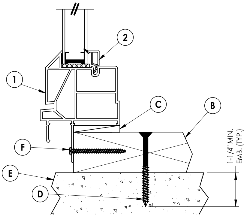
2 VERTICAL CROSS SECTION 2 2X Buck Masonry Construction
